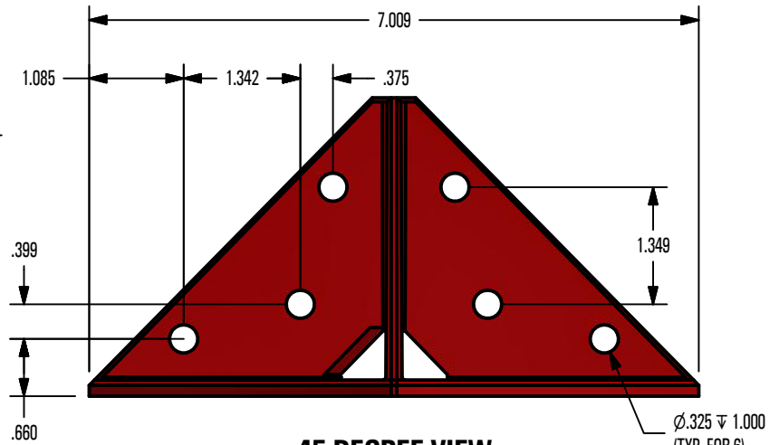
45 DEGREE VIEW
