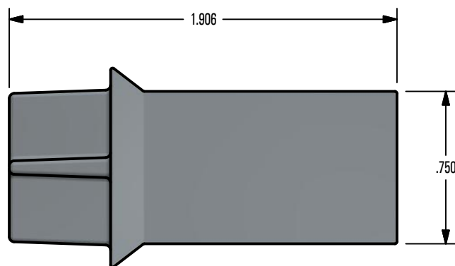
RIGHT VIEW
