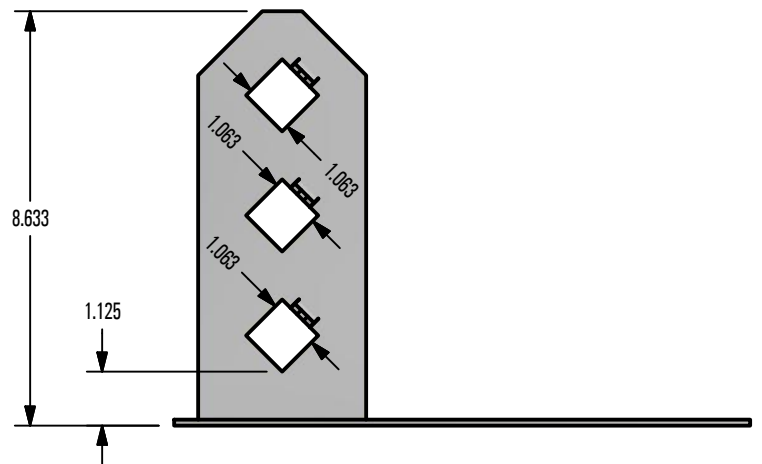
RIGHT VIEW
