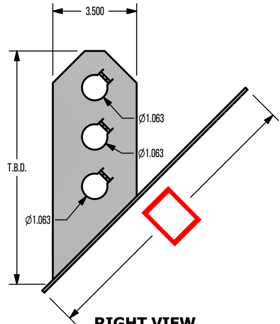
RIGHT VIEW
