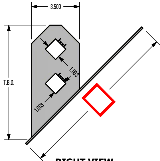
RIGHT VIEW
