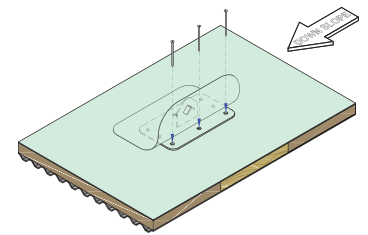
Pre-Skirted Target Patch New Construction Option
