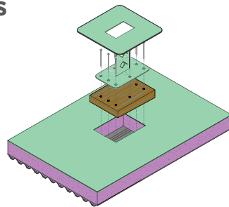
Wood Blocking Retrofit Option
