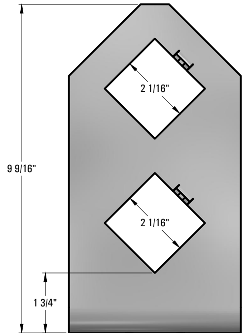
RIGHT VIEW
