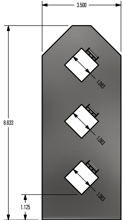
RIGHT VIEW
