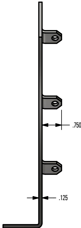
FRONT VIEW
