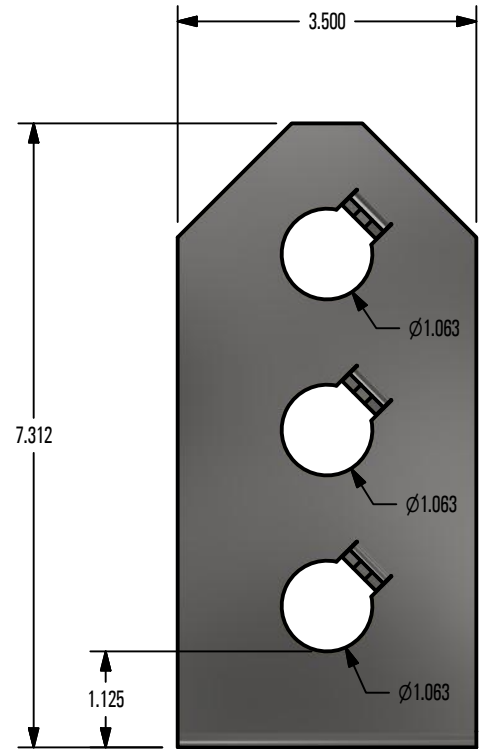
RIGHT VIEW
