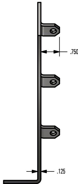
FRONT VIEW
