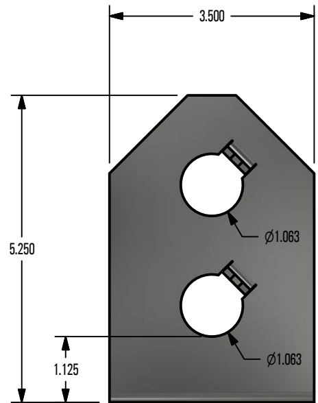
RIGHT VIEW
