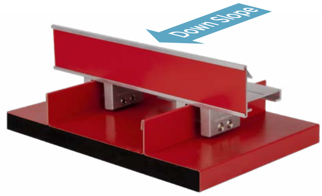
Typical 2" iClad-S™ Assembly
